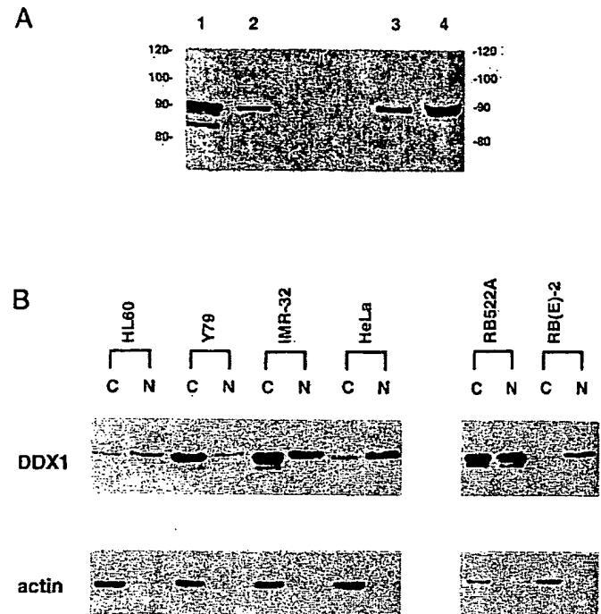
FIG. 8. Distribution of DDX1 in the nucleus and cytoplasm. A, cytosolic and nuclear extracts were prepared from RB522A and electrophoresed in a 7% SDS-PAGE gel. Cytosolic extracts were loaded in lanes 1 (20 \mu g of protein) and 2 (10 \mu g), while nuclear extracts were loaded in lanes 3 (10 \mu g) and 4 (20 \mu g). DDX1 was visualized using a 1:5000 dilution of the antiserum to the N terminus. The BenchMark protein ladder size markers (kilodaltons) are indicated on the left. B, cytosolic and nuclear extracts were prepared from HL60, Y79, IMR-32, HeLa, RB522A, and RB(E)-2 and electrophoresed in an 8% SDS-PAGE gel. Twenty \mu g of proteins were loaded in each lane marked C (cytosolic) and N (nuclear). DDX1 was visualized using a 1:5000 dilution of the antiserum to the N terminus. Actin levels were analyzed using a 1:200 dilution of anti-actin antibody (Santa Cruz Biotechnology).
